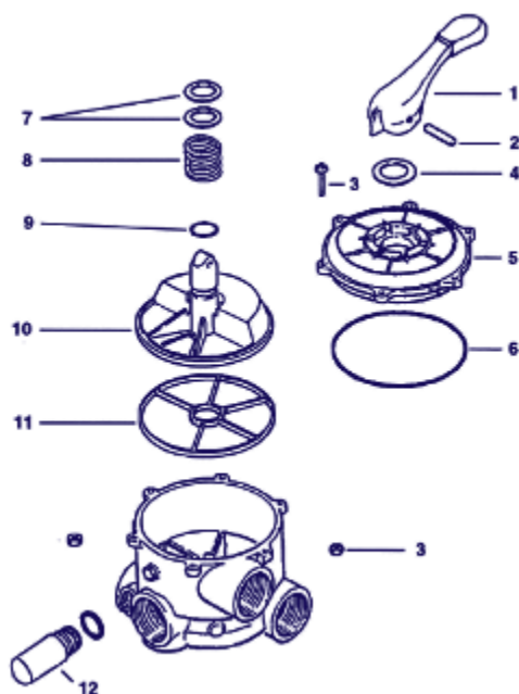
VANNE SIDE
